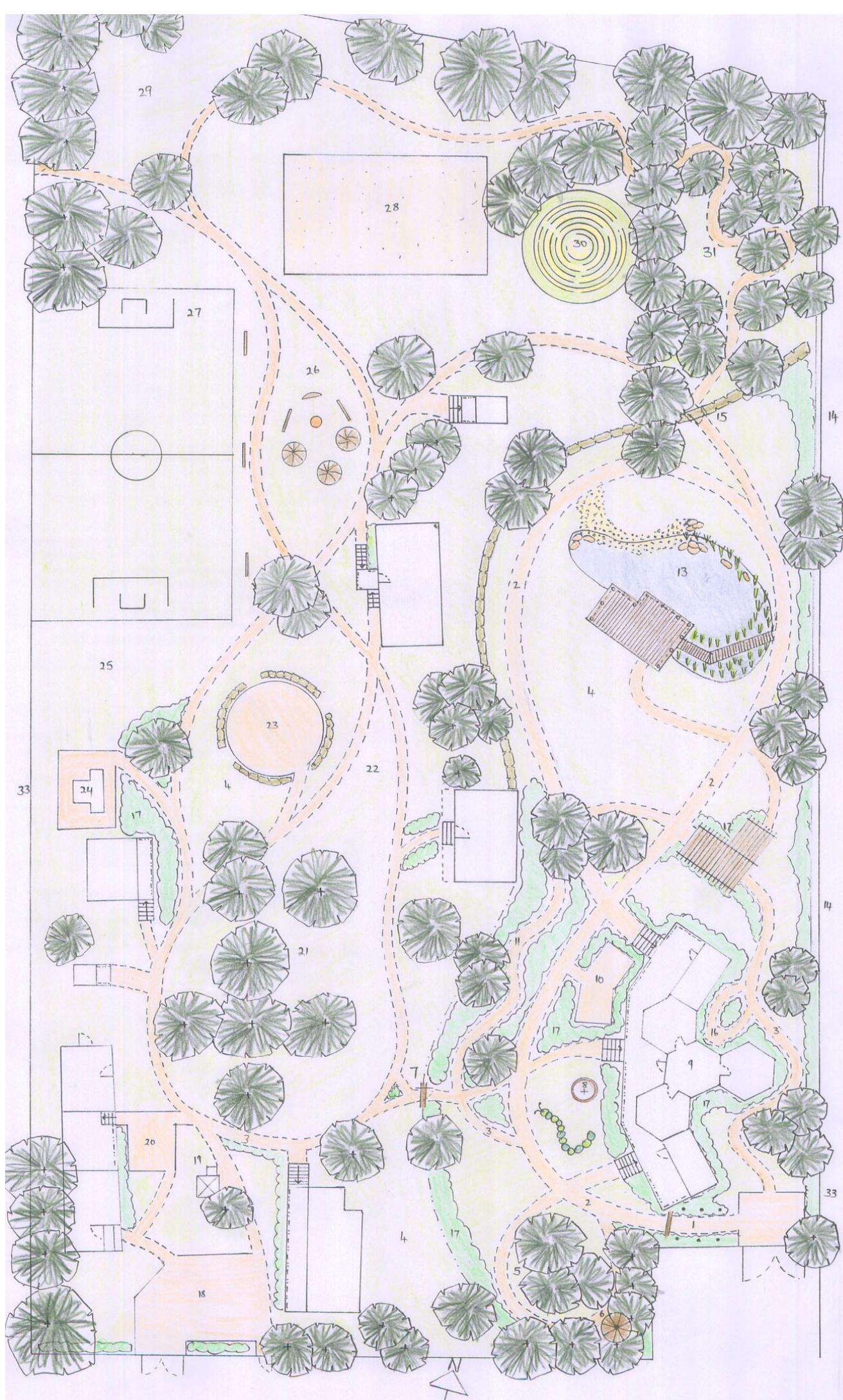
The Stork Centre And Summercamp Site Plan 1:250
